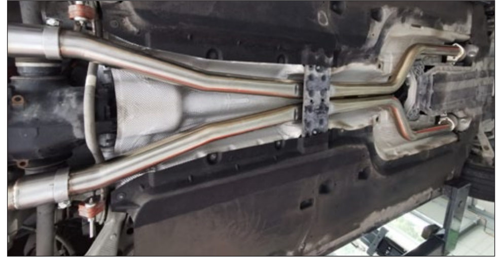
Middle pipes without muffler
