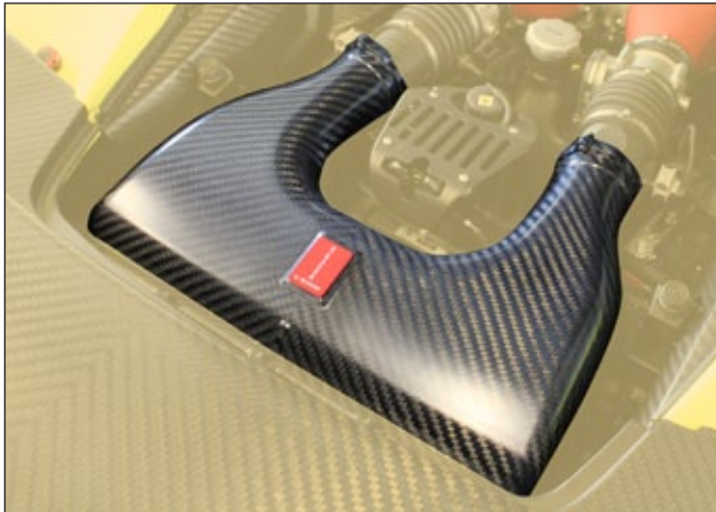
Airbox cover ..... 458 000 17 with logo, visible carbon fibre glossy* 4 parts set
